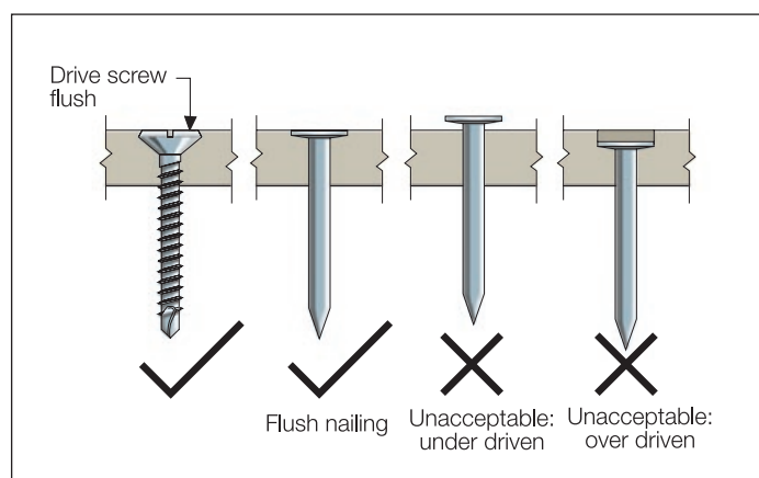
FIGURE 6 FASTENER DEPTH
